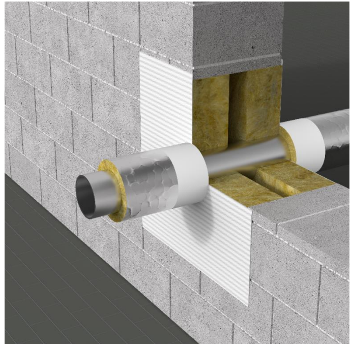
Figure 4.1: Fire rated pain INTU FR COAT A application
