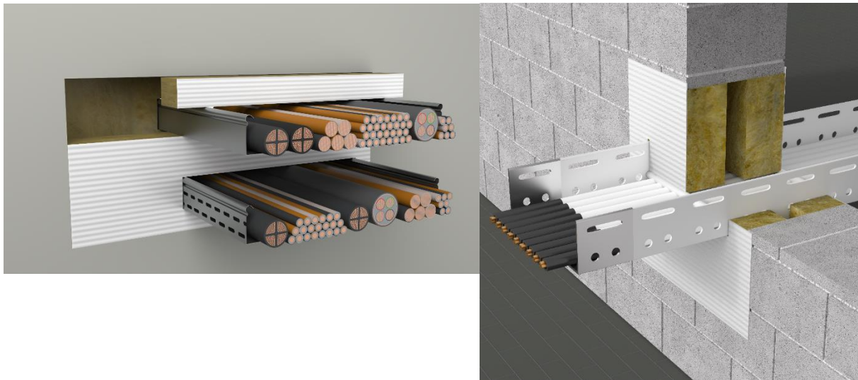
Figure 4.2: Fire rated board INTU FR UNIBOARD application
