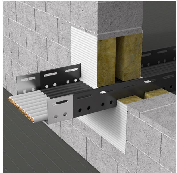
Figure 4.1: Fire rated ablative board INTU FR BOARD A application
